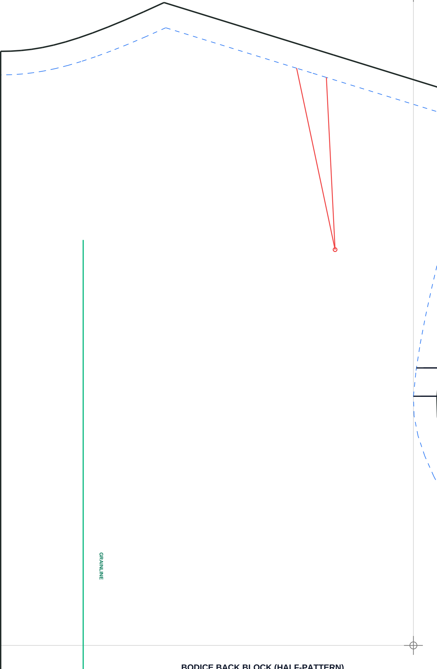
BODICE BACK BLOCK (HALF-PATTERN)
